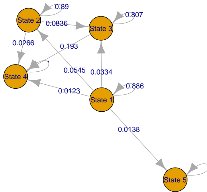
Figure 8: Another example of plot.hmm .
